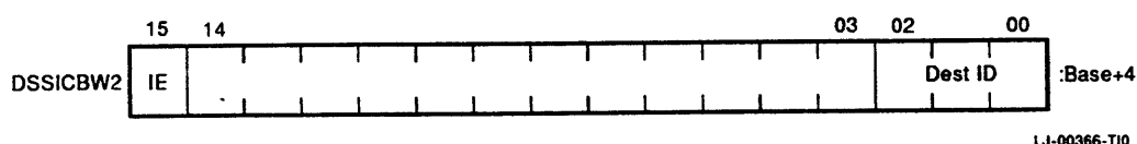
Figure 3-75 DSSI Command Block word 2
