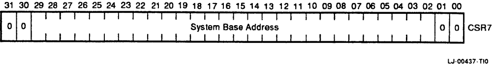
Figure 3-49 CSR7 Format
