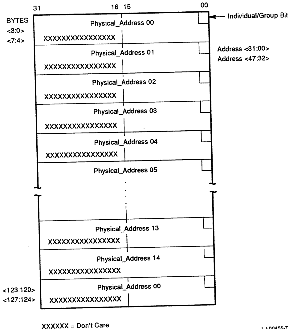
Figure 3-56 Perfect Filtering Setup Frame Buffer Format
