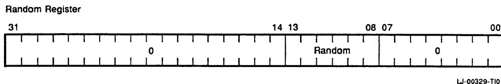
Figure 3-6 Random Register
