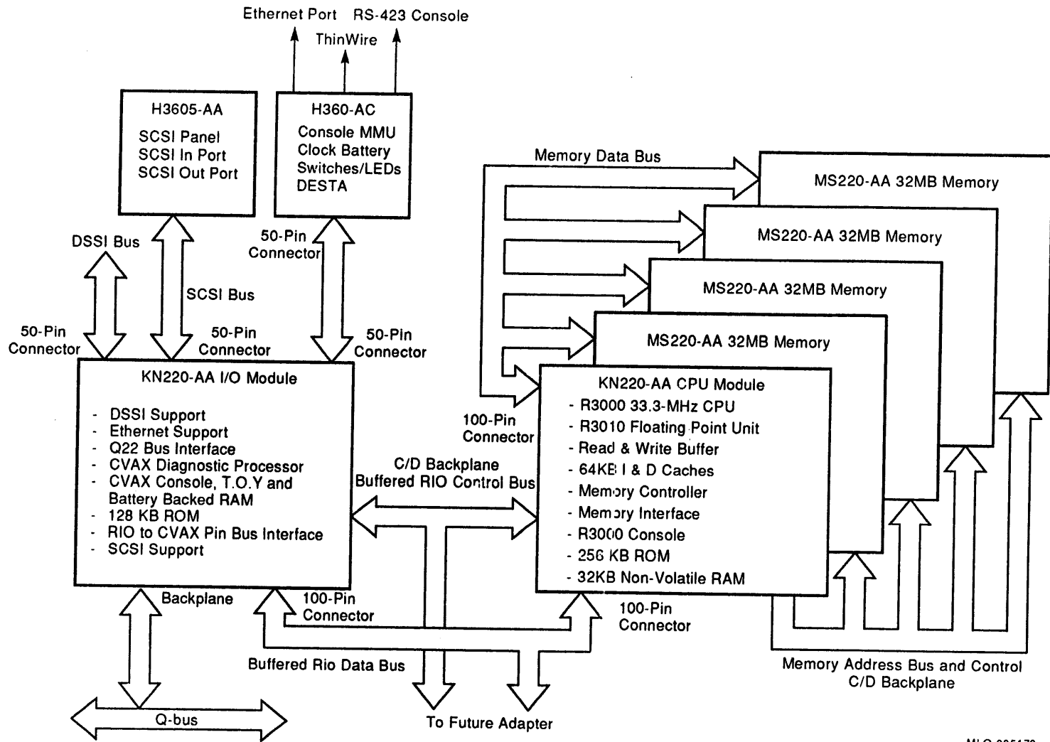
Figure 1-3 DECSYSTEM 5500 Block Diagram
