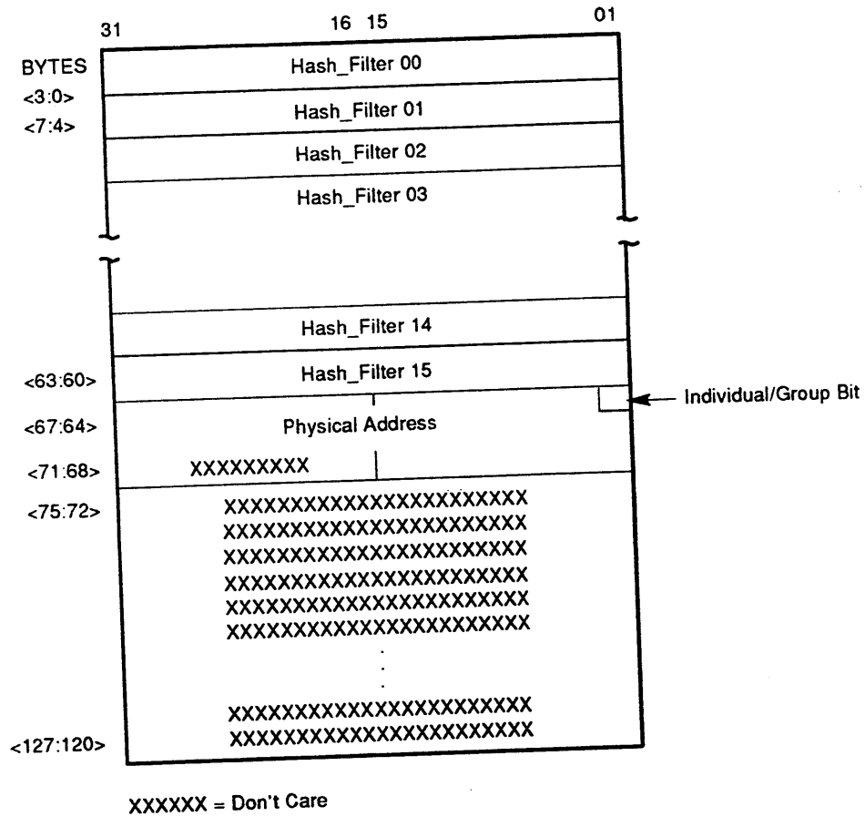
Figure 3-57 Imperfect Filtering Setup Frame Format
