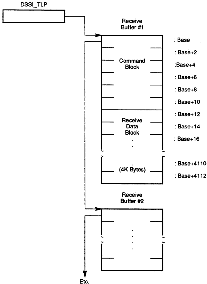
Figure 3-69 Receive Buffers
