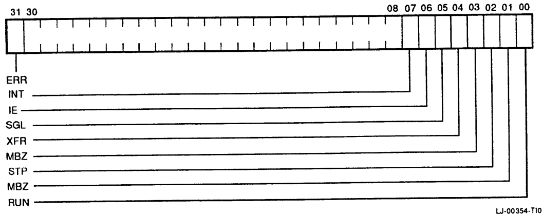
Figure 3-37 Timer Control Registers
