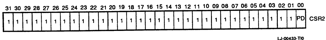
Figure 3-45 CSR2 Format
