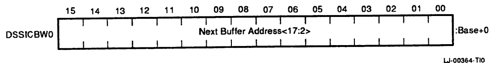
Figure 3-73 DSSI Command Block Word 0
