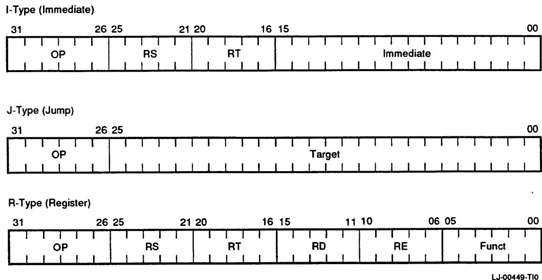
Figure 3-1 R3000 Instructions
