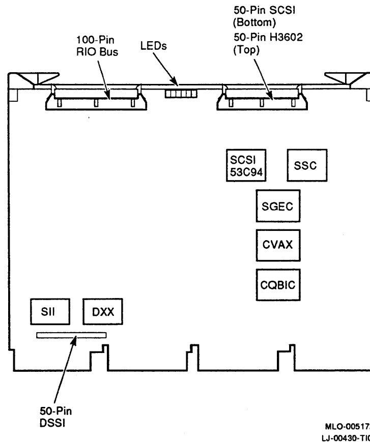
Figure 1-5 KN220-AA I/O Module Layout
