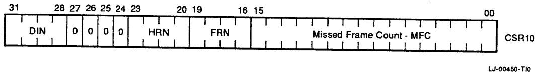
Figure 3-51 SGEC Identification and Missed Frame Count Format
