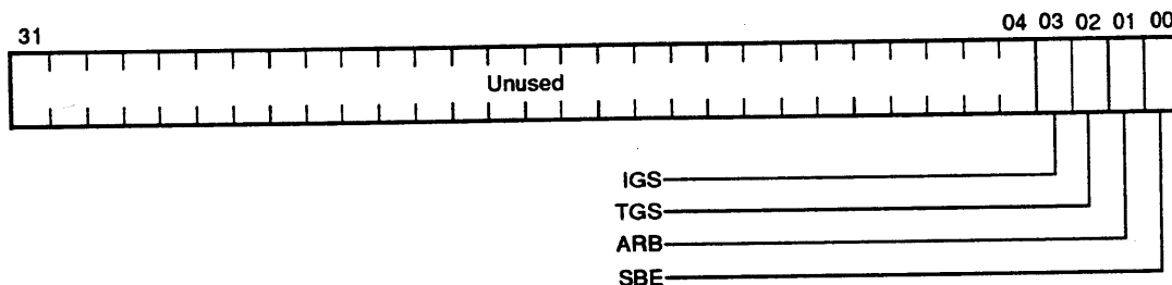
Figure 3-86 DSSI Diagnostic Register 2
