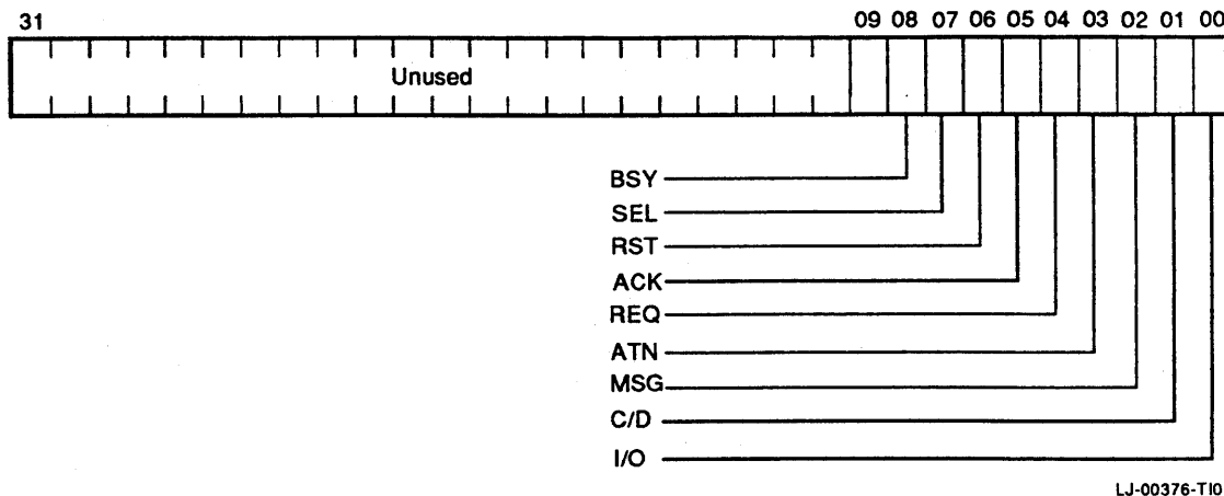
Figure 3-85 DSSI Diagnostic Register 1
