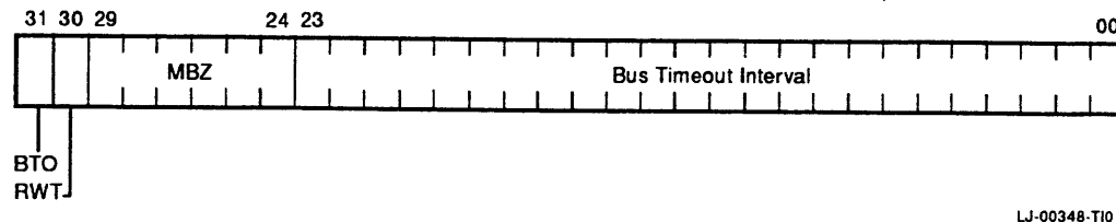
Figure 3-27 CDAL Bus Timeout Control Register
