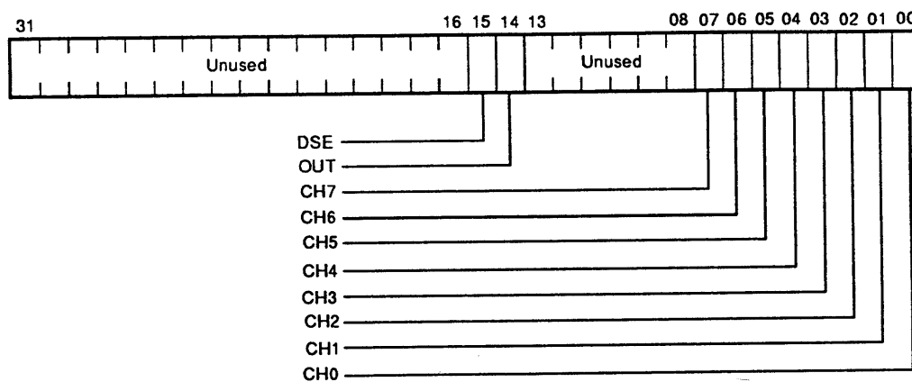
Figure 3-77 DSSI Control Register
