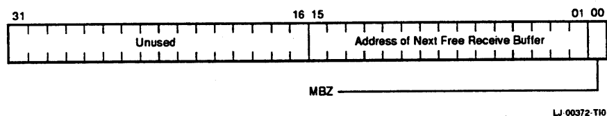
Figure 3-81 DSSI Target List Pointer Register
