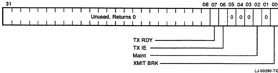
Figure 3-33 Console Transmitter Control/Status Register
