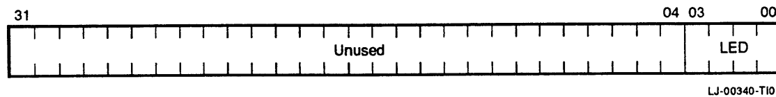
Figure 3-17 R3000 LED Register
