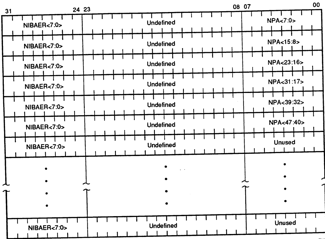
Figure 3-42 Network Interface Station Address ROM
