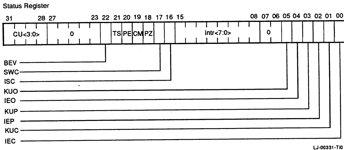
Figure 3-8 Status Register
