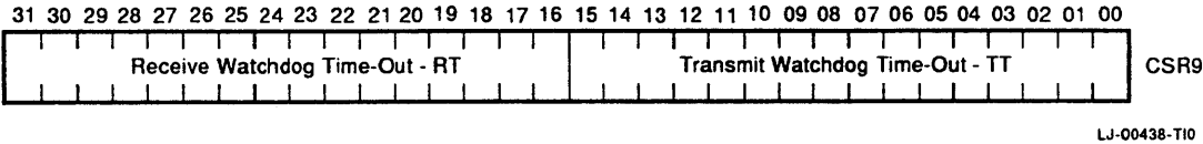
Figure 3-50 CSR9 Format
