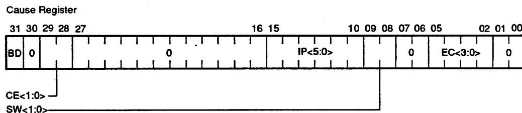
Figure 3-7 Cause Register
