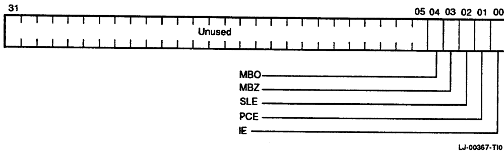
Figure 3-76 DSSI Control/Status Register
