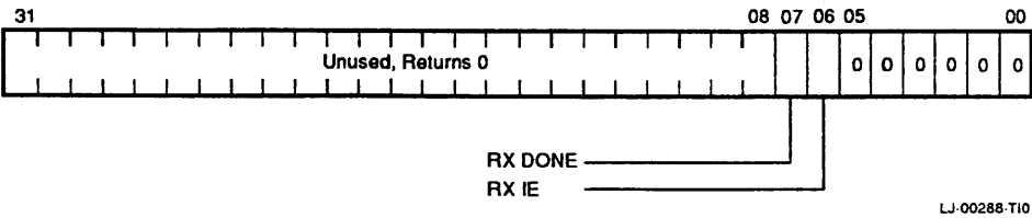
Figure 3-31 Console Receive Control/Status Register
