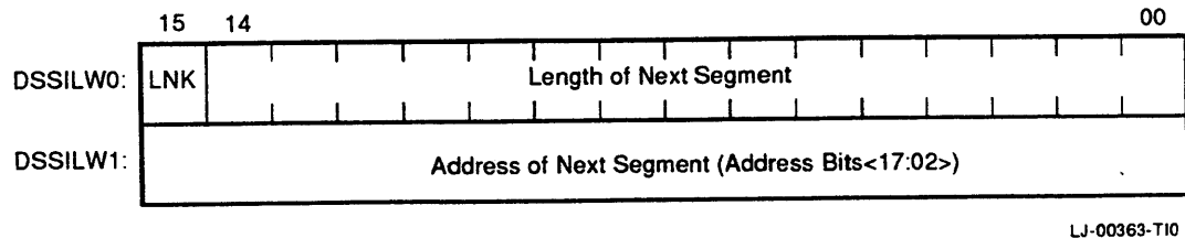
Figure 3-70 Transmit Data Segment Link
