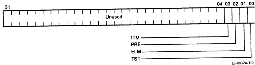
Figure 3-83 DSSI Diagnostic Control Register
