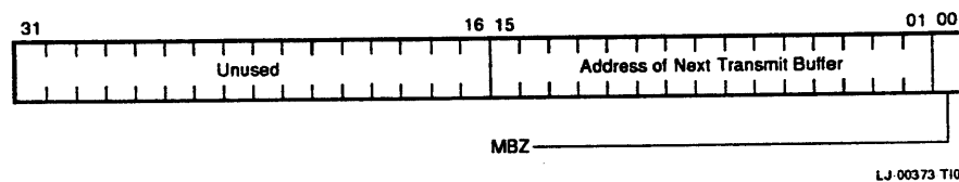
Figure 3-82 DSSI Initiator List Pointer Register
