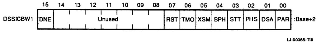
Figure 3-74 DSSI Command Block Word 1
