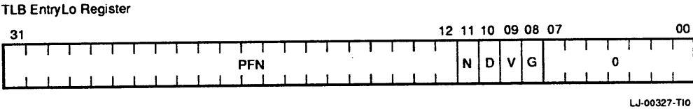
Figure 3-4 TLB EntryLo Register
