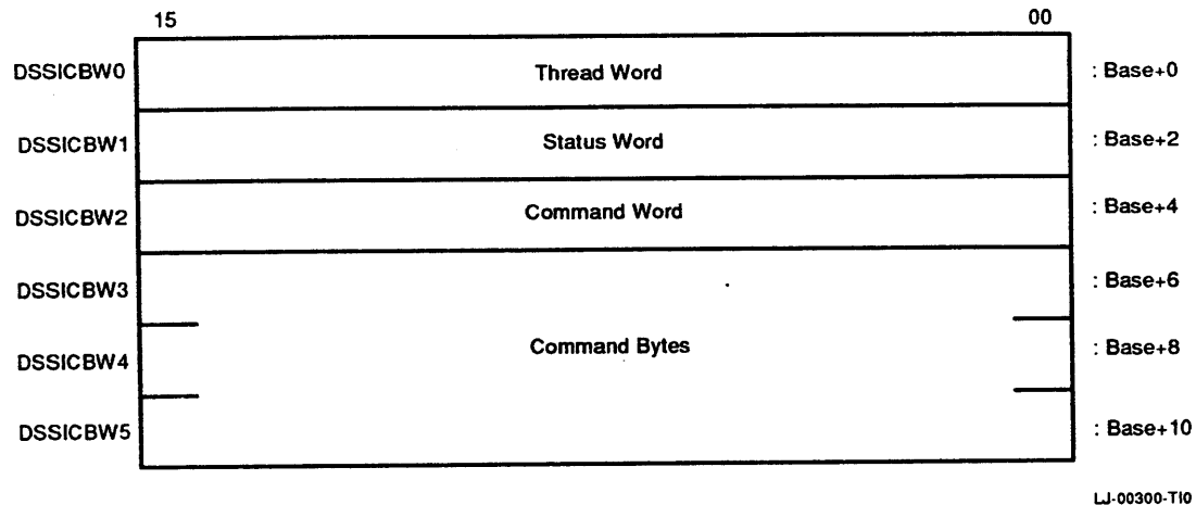
Figure 3-72 DSSI Command Block
