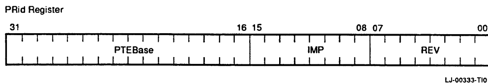
Figure 3-10 Processor Revision Identifier Register
