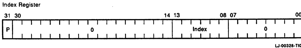
Figure 3-5 Index Register
