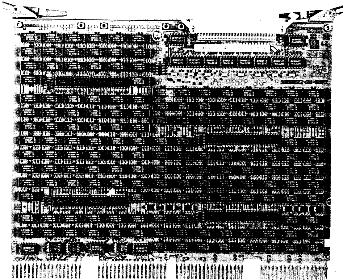
Figure 1-6 MS220-Ax Memory Module
