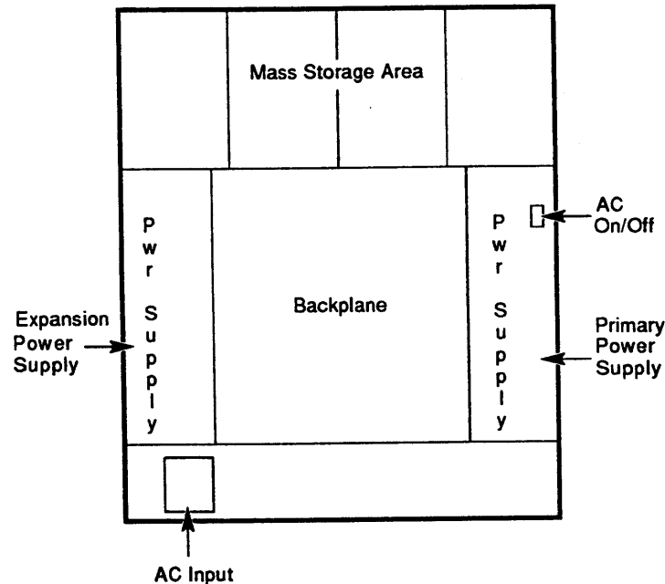
Figure 5-14 BA213 Enclosure Front View
