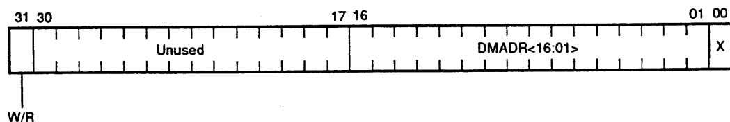
Figure 3-88 DMA Address Register
