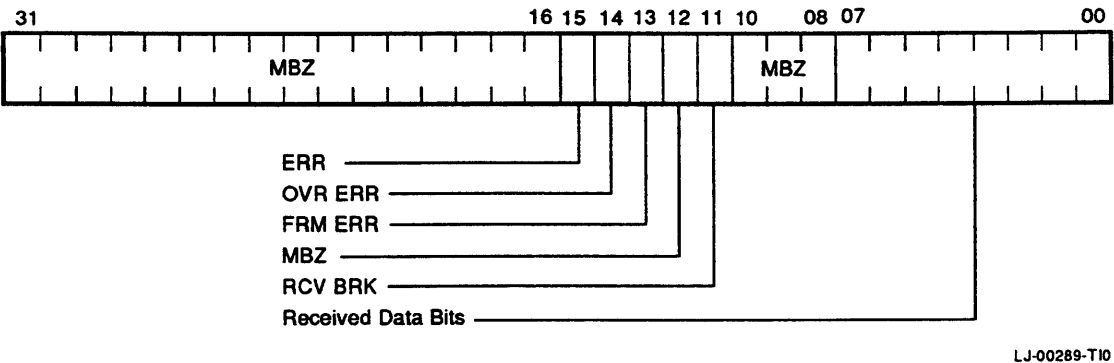
Figure 3-32 Console Receiver Data Buffer
