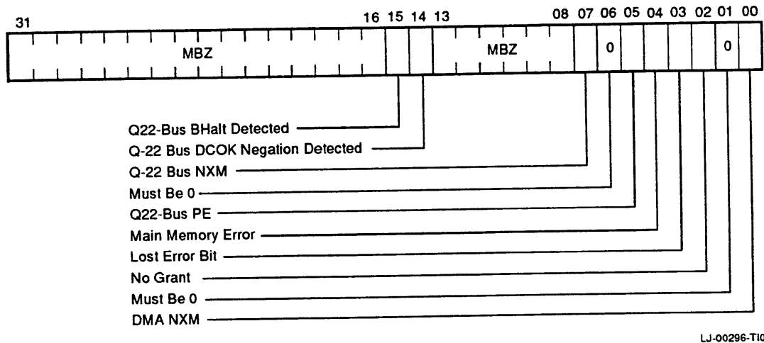
Figure 3-64 DMA System Error Register
