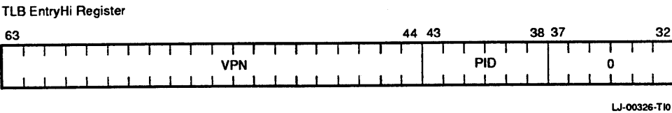
Figure 3-3 TLB EntryHi Register
