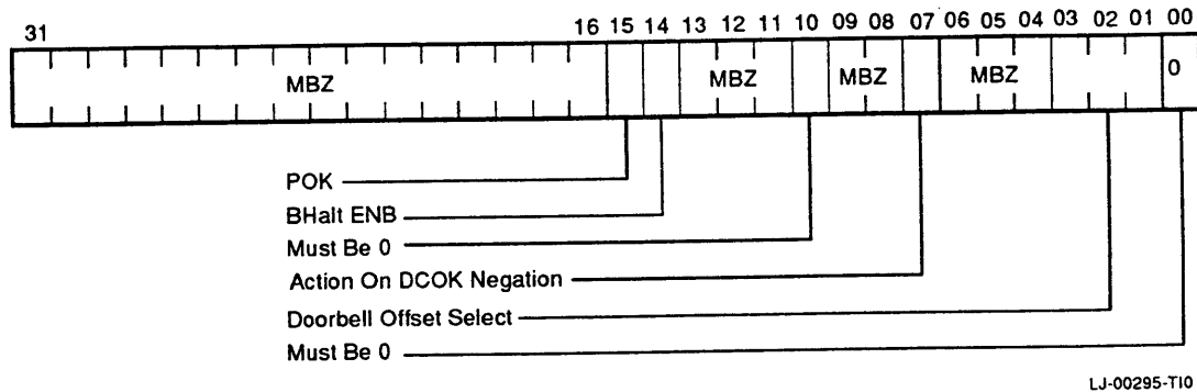
Figure 3-63 System Configuration Register
