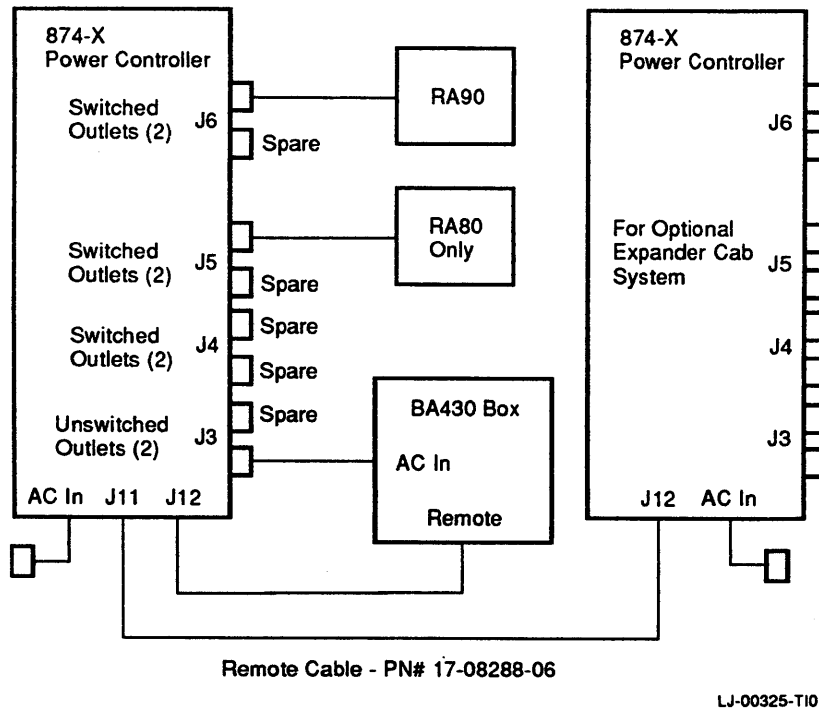
Figure 5-2 BA430-Bx System Enclosure Interconnections
