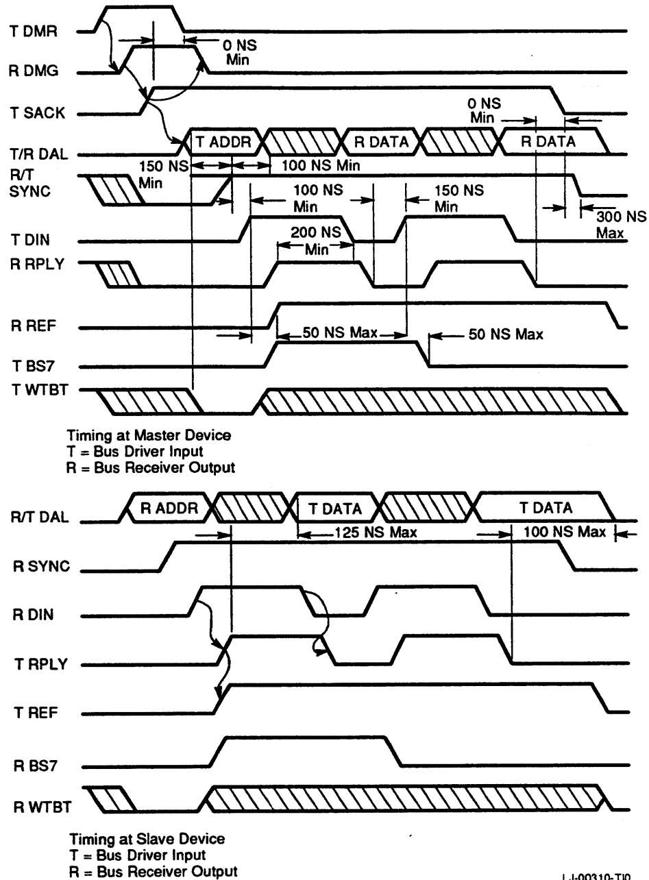
Figure A-9 DATBI Bus Cycle Timing
