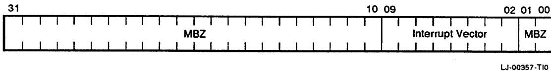
Figure 3-40 Timer Interrupt Vector Registers
