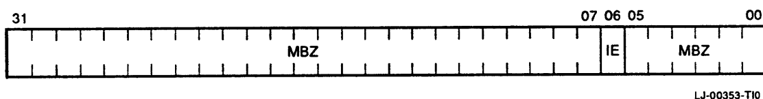
Figure 3-36 Interval Clock Control/Status Register
