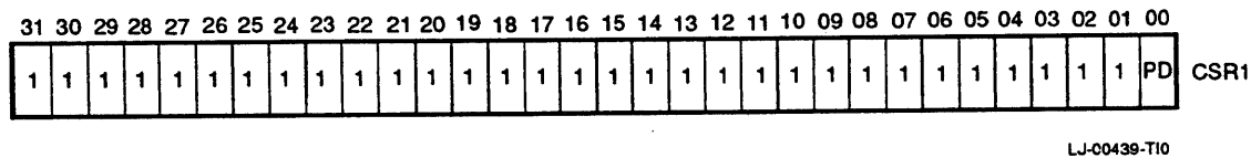
Figure 3-44 CSR1 Format
