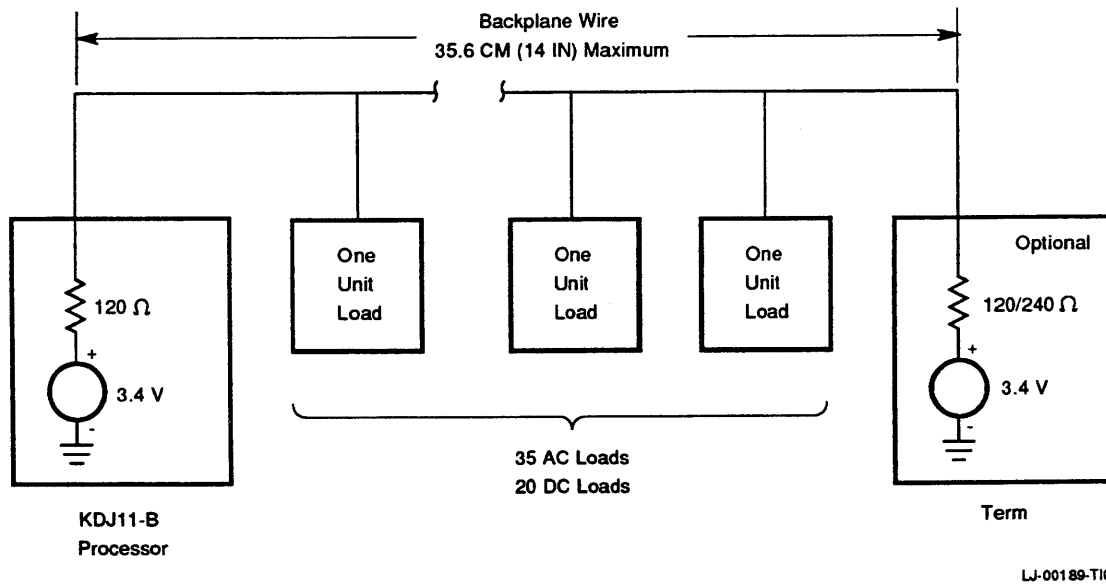
Figure A-16 Single-Backplane Configuration
